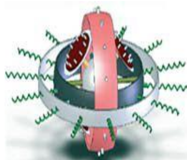
Al bio-nanorobot
